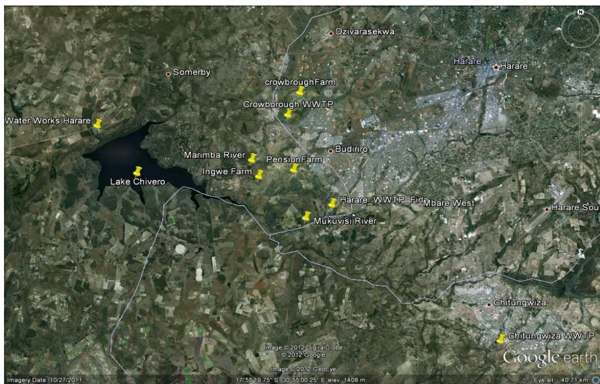
Figure 3: Google Earth Map showing the layout of wastewater treatment plants in Harare, Zimbabwe
